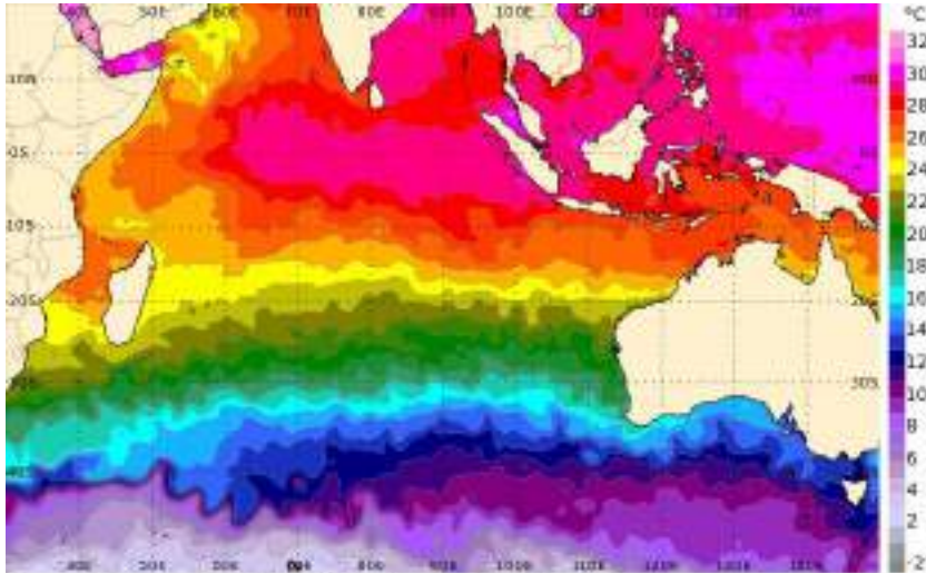
Sea surface temperature (deg C): Daily analysis for Tue 9 Sep 2025 (c) Copyright Australian Bureau of Meteorology | GANSSA
