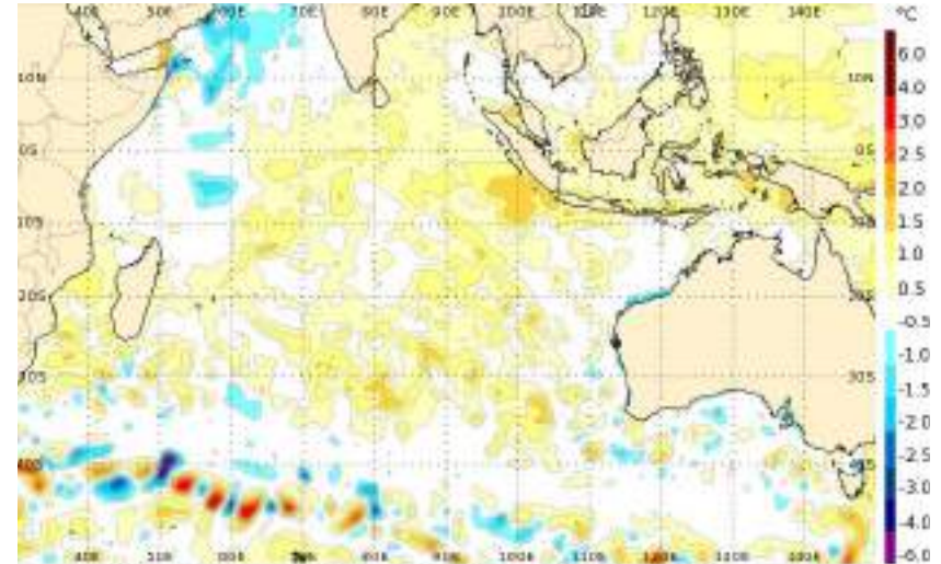
Sea surface temperature anomaly (deg C): Daily analysis for Tue 9 Sep 2025 (c) Copyright Australian Bureau of Meteorology | GANSSA | Climatology 1961-1990
